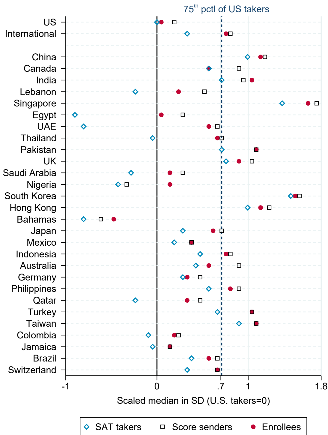
Figure 9: SAT median in standard deviations for test takers, score senders, and enrollees
