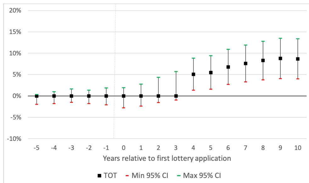
Figure 1: Cumulative effects on probability of having registered to vote, by year since first lottery
